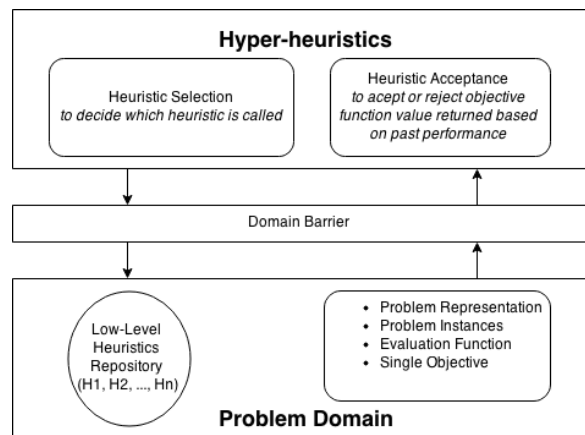
Fig. 1: Hyper-heuristics Conceptual Framework [9]
